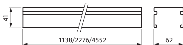
IP20/IP54-Tragschiene LL512T.../LL523X.../LL546T...
