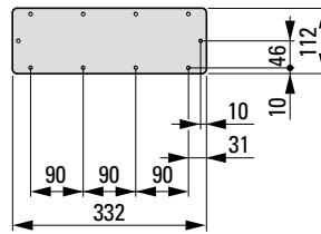
SFP-112X332-CS
